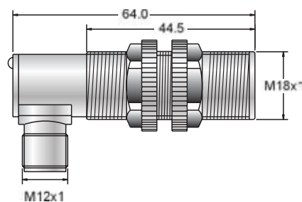
Y-state, Right Angle with QD connector Euro-style.
