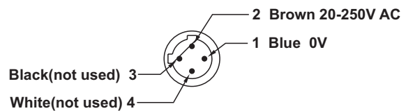
Connector pin position (Micro-style)
