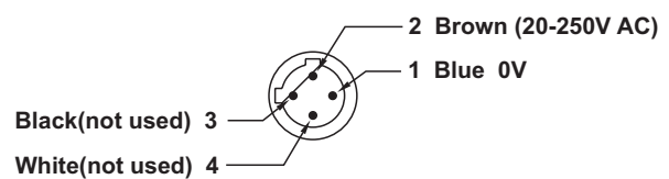
Connector pin position (Micro-style)
