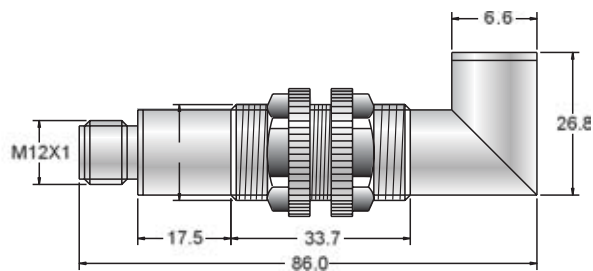
Y-state, Right Angle with QD connector Euro-style.
