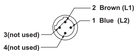
Connector pin position (Micro-style)
